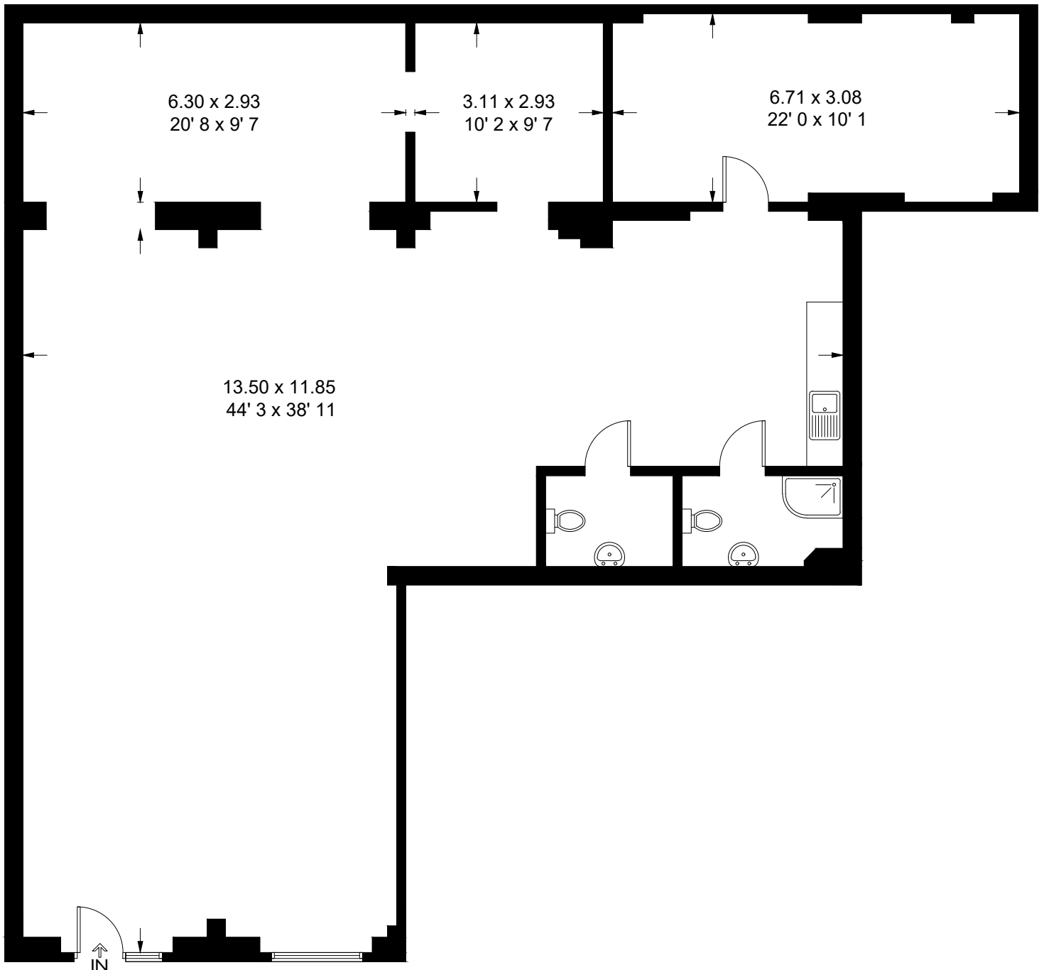
Ground Floor
